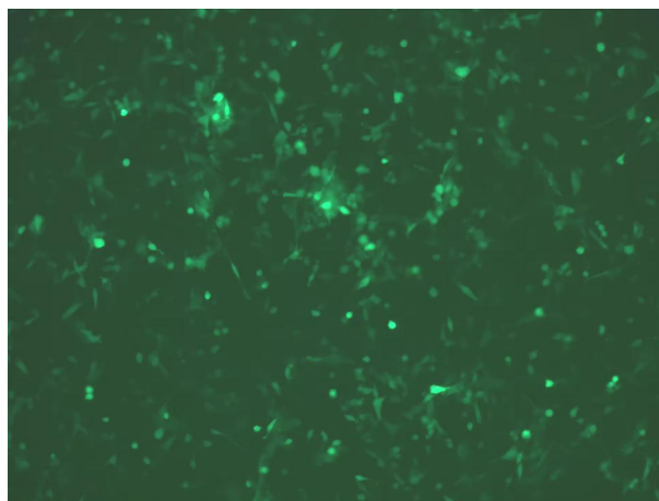
MC38-ggaOVAL-100X
